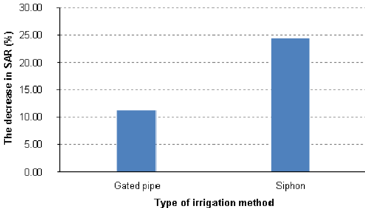
Figure 5. The sodium ratio for both treatments.
